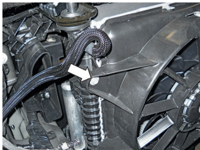
LH mounting bolt
