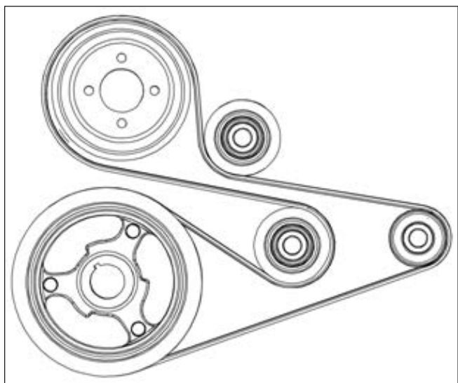
42. Remove the three (3) bolts (10 mm socket) securing the water pump pulley to the engine and remove the water pump pulley.
